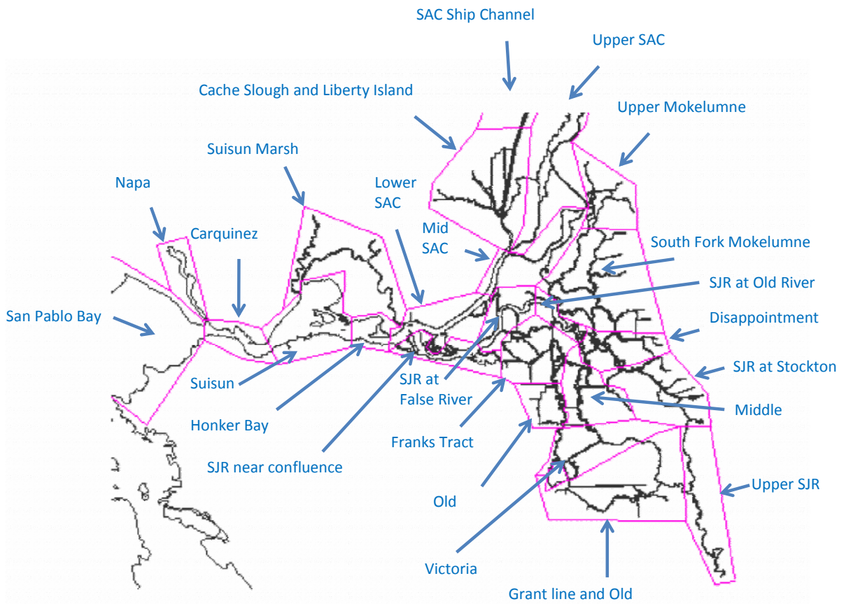
Figure 41 Source regions.
