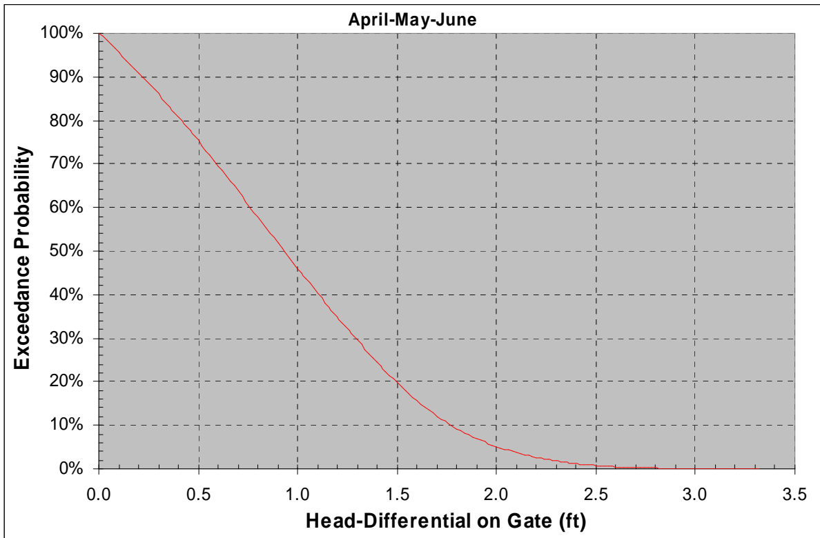
Figure 3.12 DSM-2 Results, Old River Gate-Closed Head-Differentials
