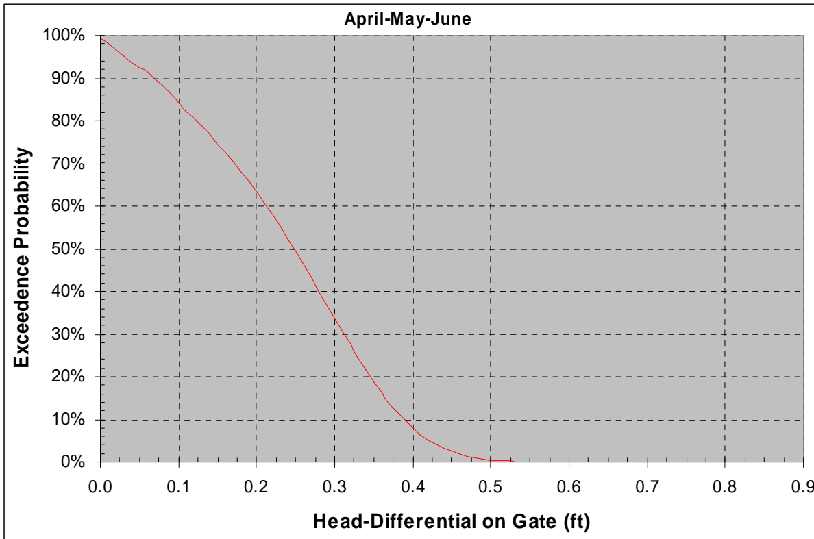
Figure 3.13 DSM-2 Results, Connection Slough Gate-Closed Head-Differentials
