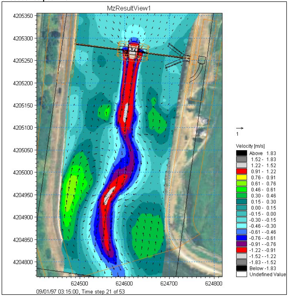
Figure 3.8 MIKE-21 Results for Old River with Gates Open, Flood Tide with ~1% exceedance peak flow.
