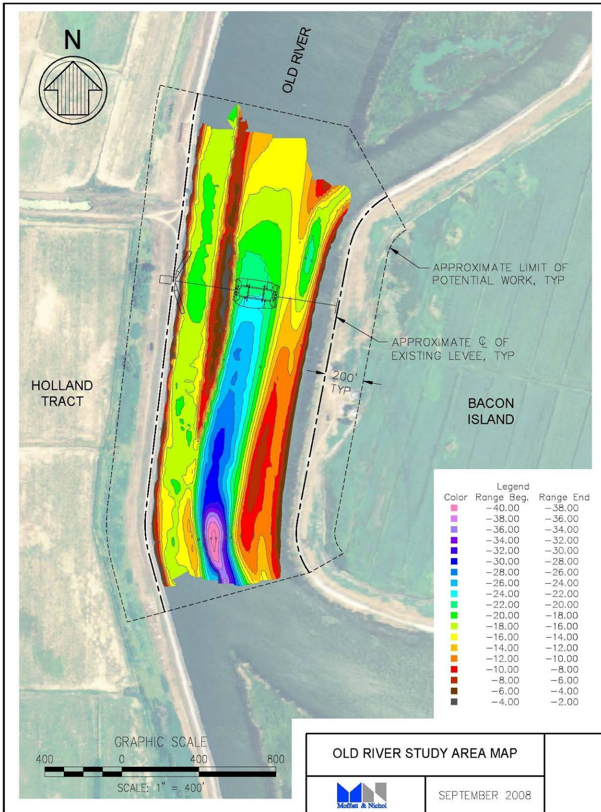
Figure 2.2 Old River Site
