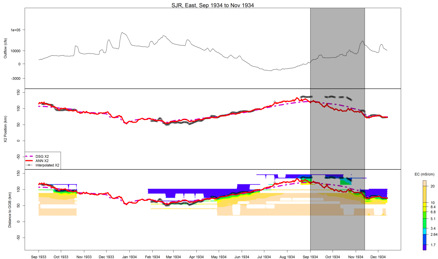
Figure B-50 Flow, X2, and salinity data for SJR, East, Sep 1934 to Nov 1934
