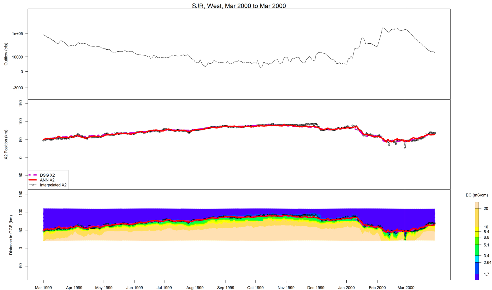
Figure B-44 Flow, X2, and salinity data for SJR, West, Mar 2000 to Mar 2000
