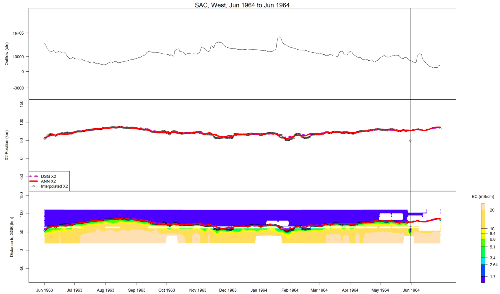
Figure B-17 Flow, X2, and salinity data for SAC, West, Jun 1964 to Jun 1964
