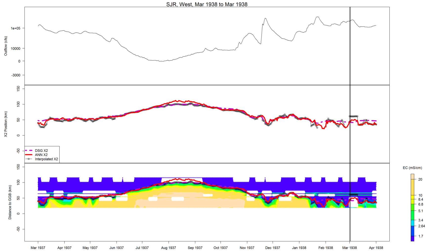
Figure B-27 Flow, X2, and salinity data for SJR, West, Mar 1938 to Mar 1938
