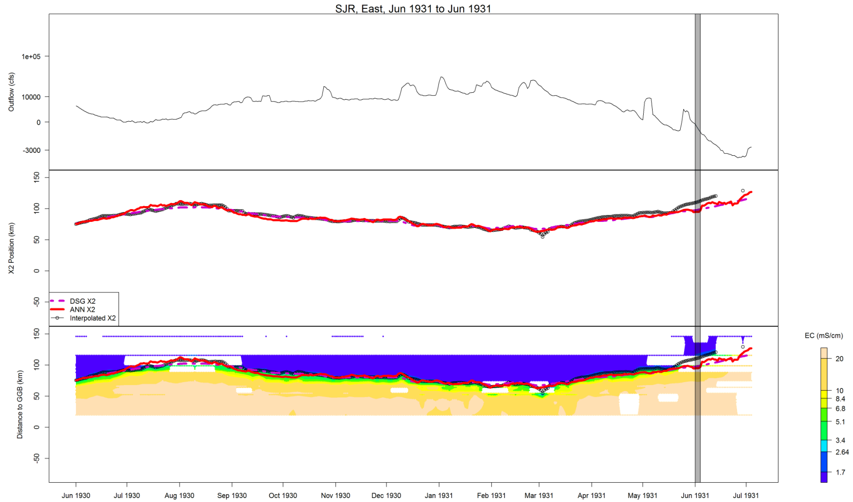
Figure B-47 Flow, X2, and salinity data for SJR, East, Jun 1931 to Jun 1931
