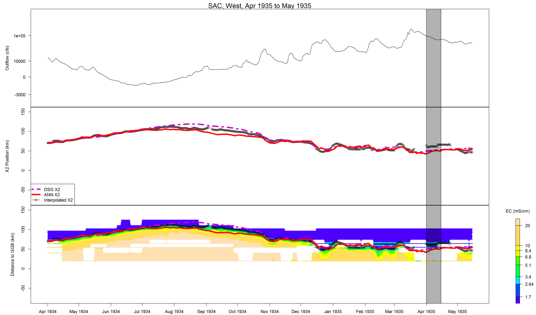
Figure B-1 Flow, X2, and salinity data for SAC, West, Apr 1935 to May 1935
