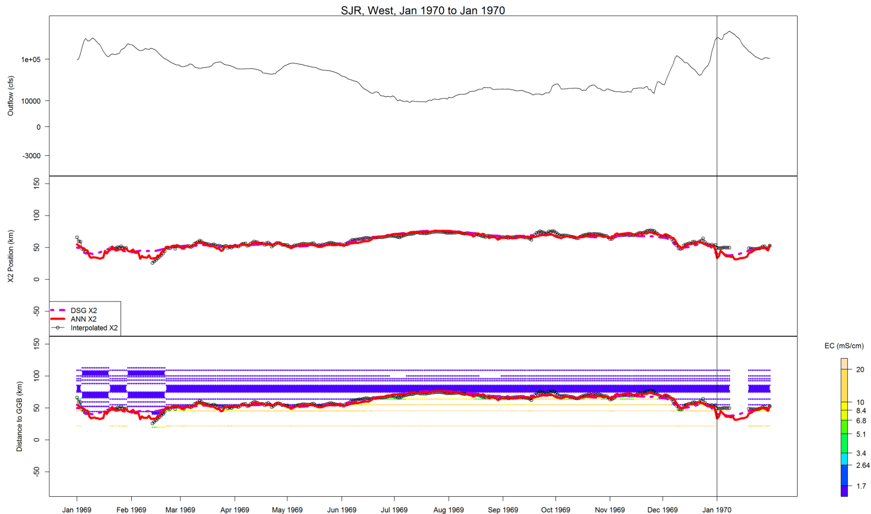
Figure B-40 Flow, X2, and salinity data for SJRW, West, Jan 1970 to Jan 1970
