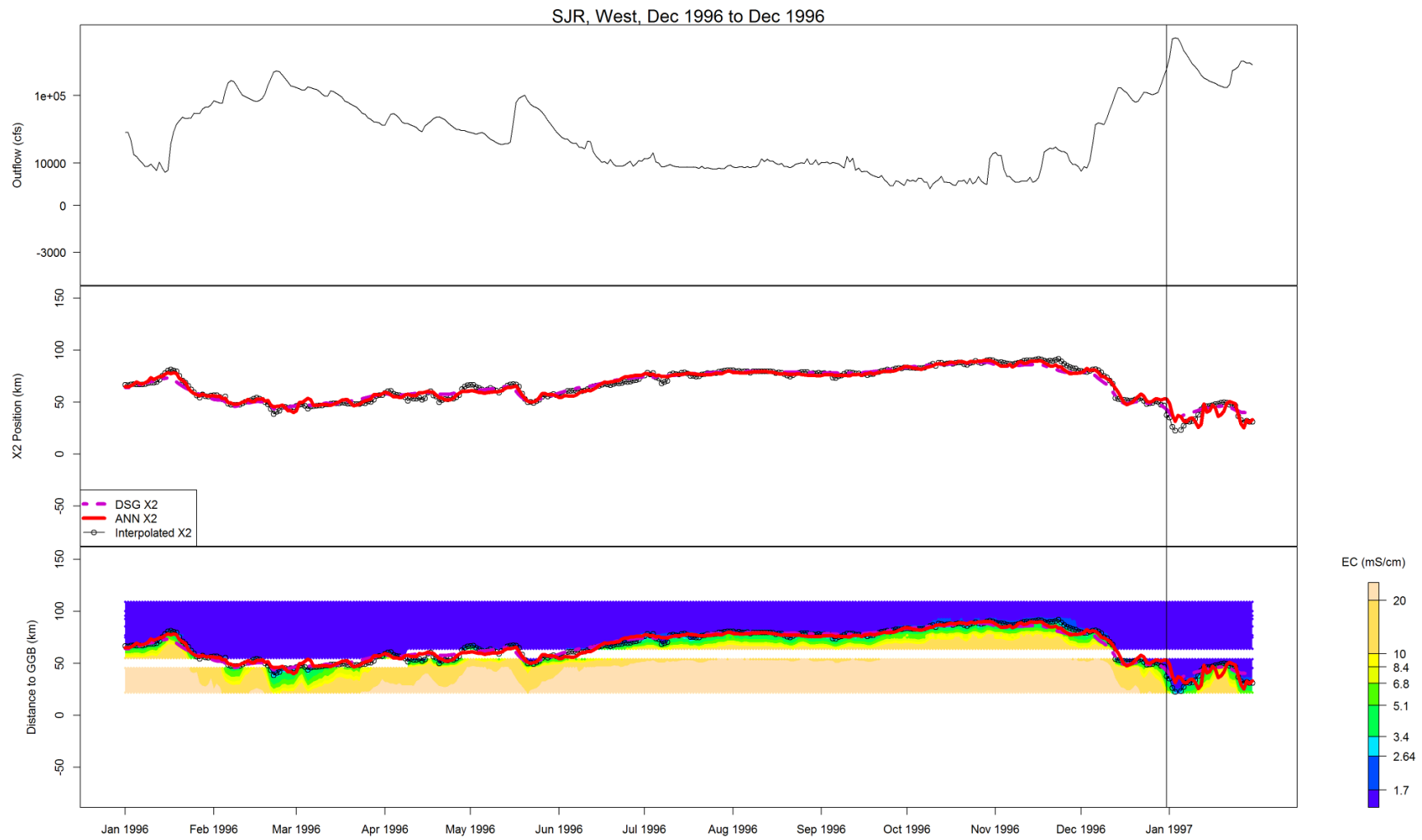
Figure B-42 Flow, X2, and salinity data for SJR, West, Dec 1996 to Dec 1996
