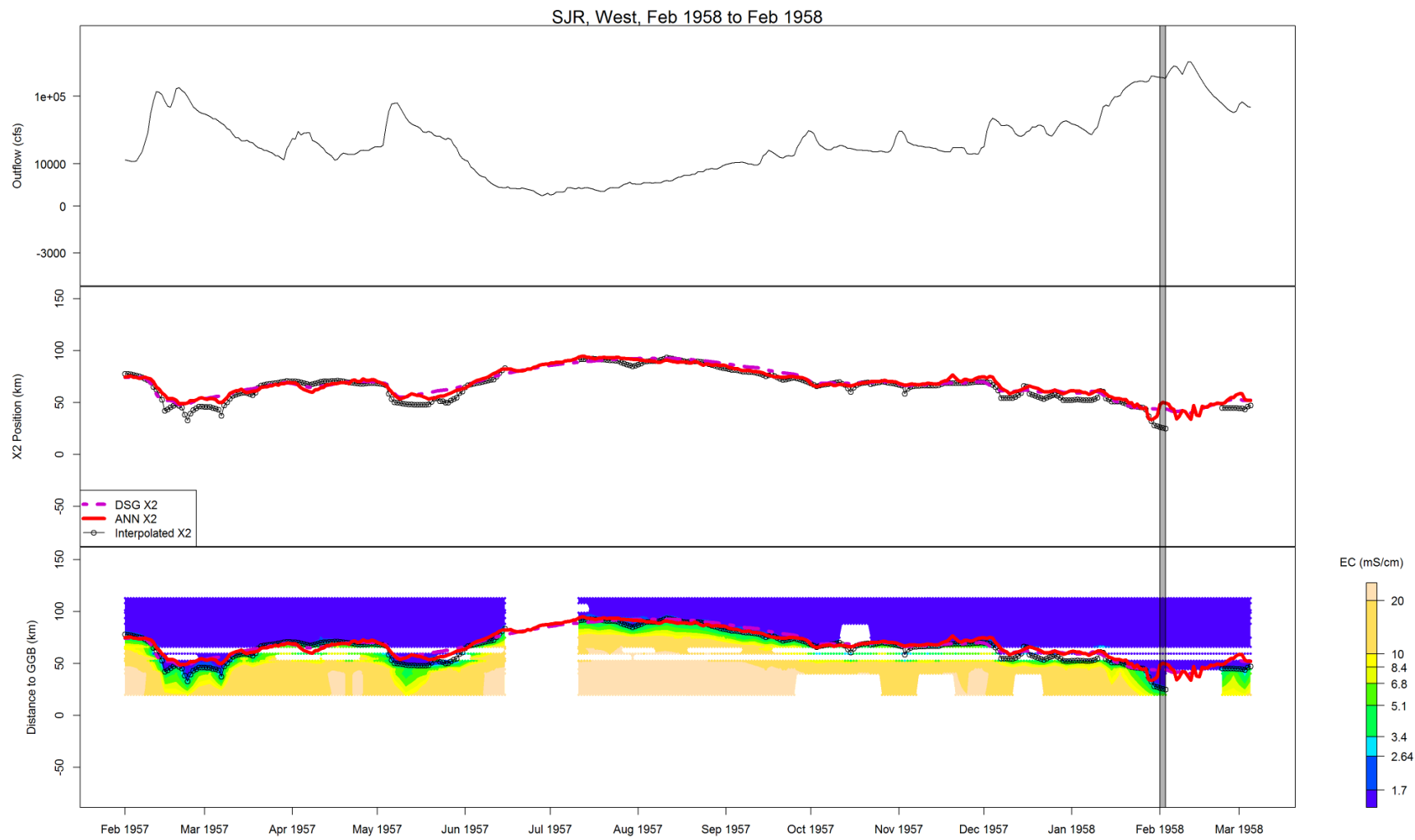
Figure B-36 Flow, X2, and salinity data for SJR, West, Feb 1958 to Feb 1958
