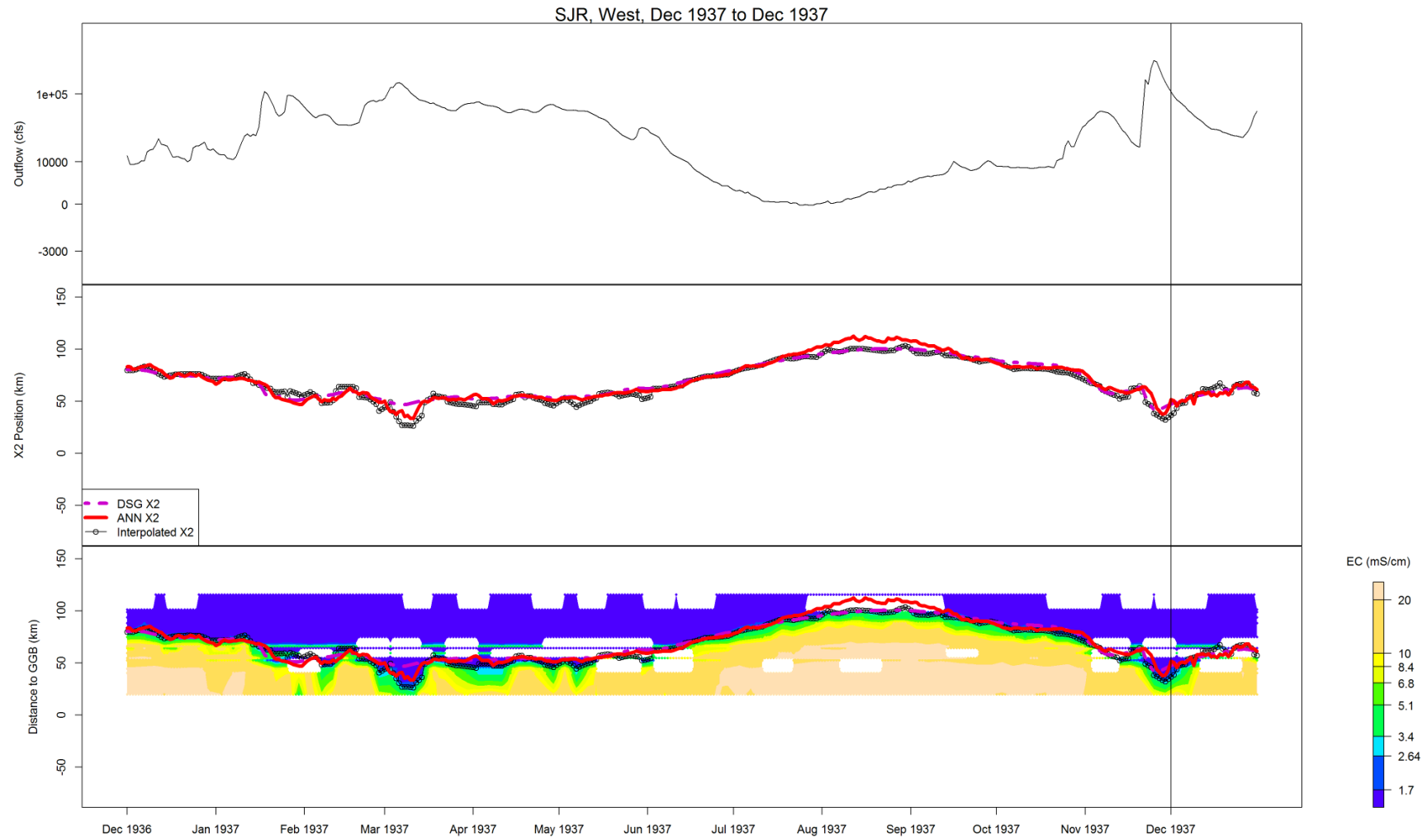
Figure B-25 Flow, X2, and salinity data for SJR, West, Dec 1937 to Dec 1937
