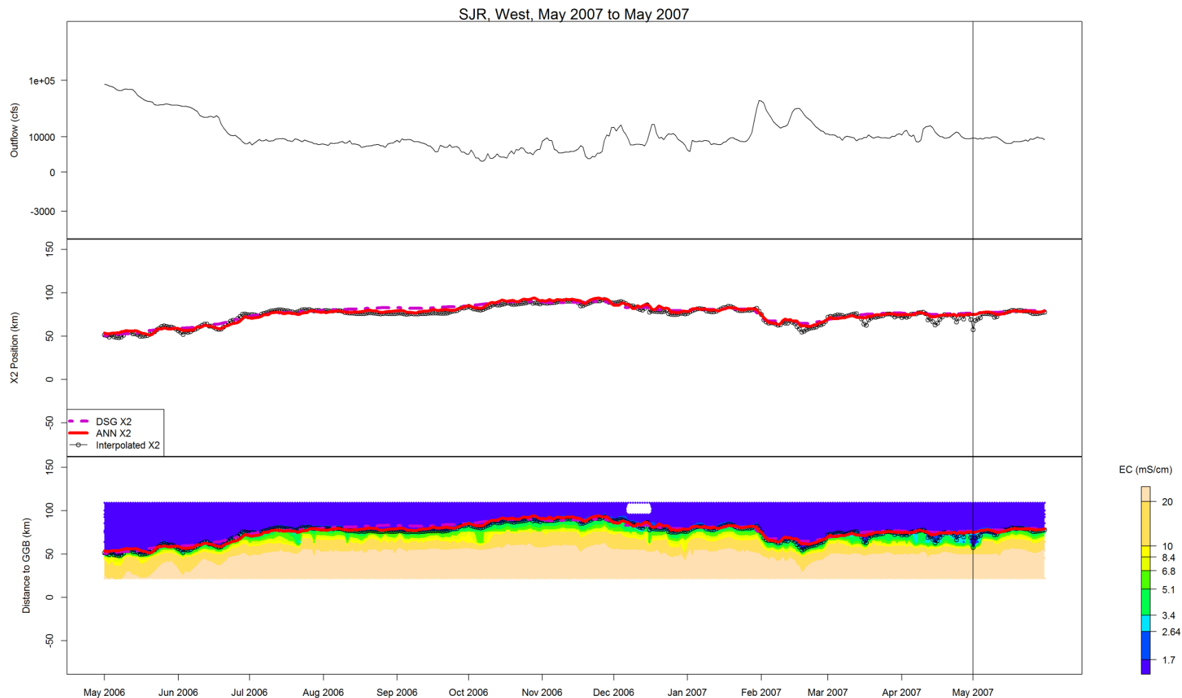
Figure B-46 Flow, X2, and salinity data for SJR, West, May 2007 to May 2007
