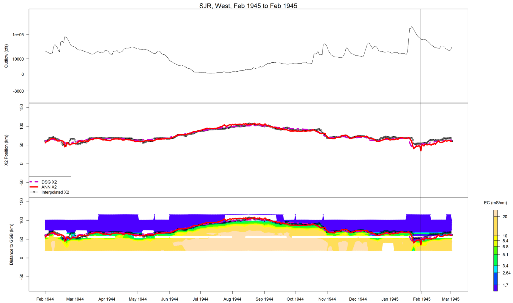
Figure B-32 Flow, X2, and salinity data for SJR, West, Feb 1945 to Feb 1945
