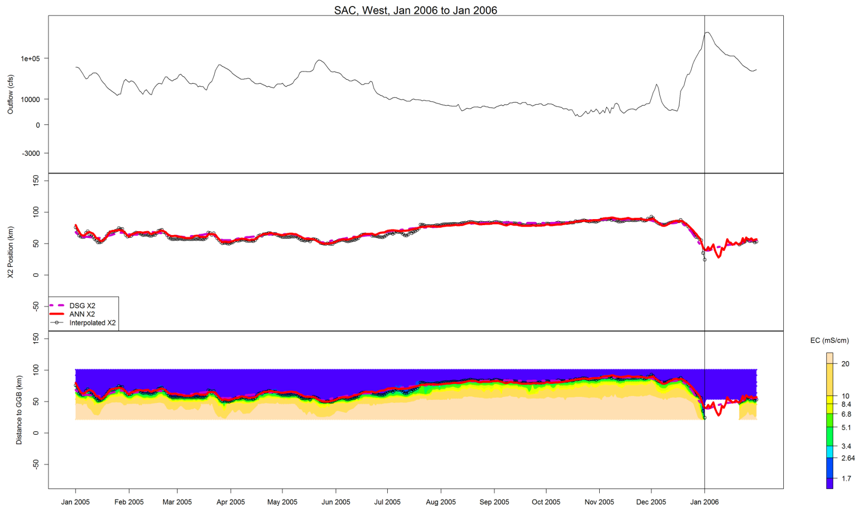
Figure B-18 Flow, X2, and salinity data for SAC, West, Jan 2006 to Jan 2006
