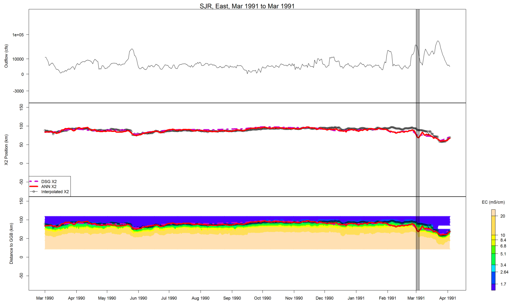
Figure B-54 Flow, X2, and salinity data for SJR, East, Mar 1991 to Mar 1991
