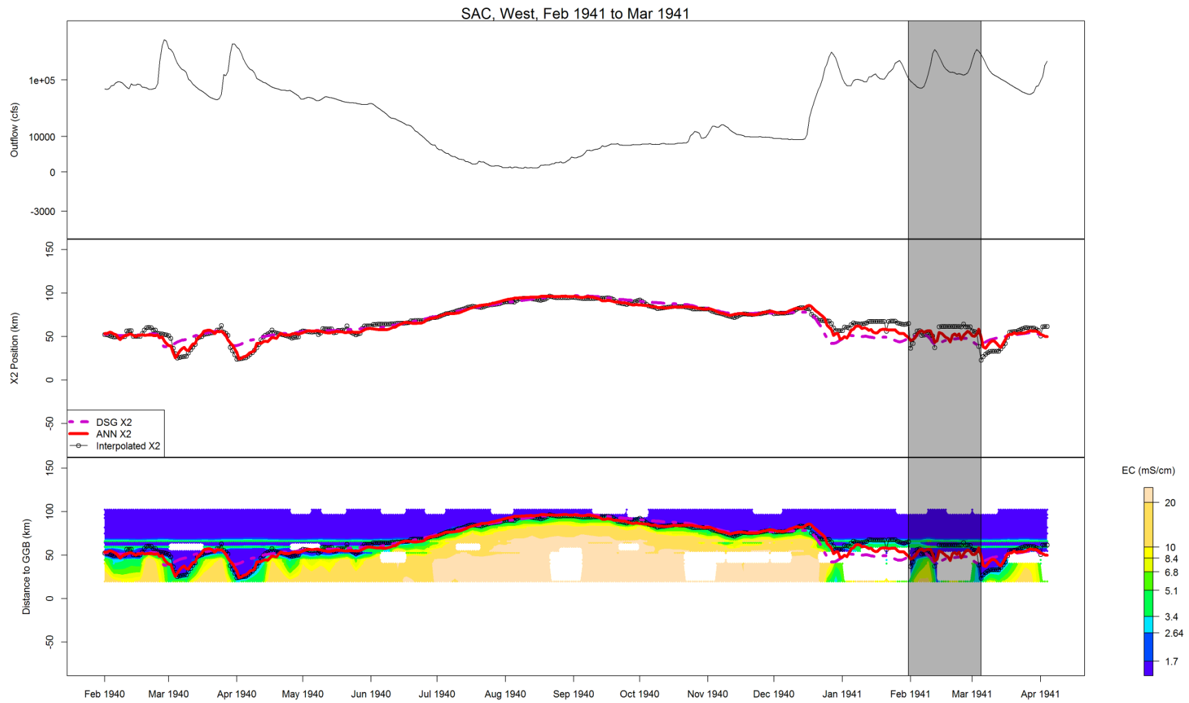
Figure B-6 Flow, X2, and salinity data for SAC, West, Feb 1941 to Mar 1941
