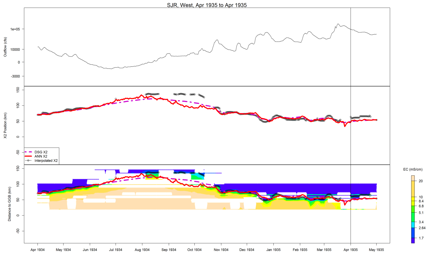
Figure B-22 Flow, X2, and salinity data for SJR, West, Apr 1935 to Apr 1935
