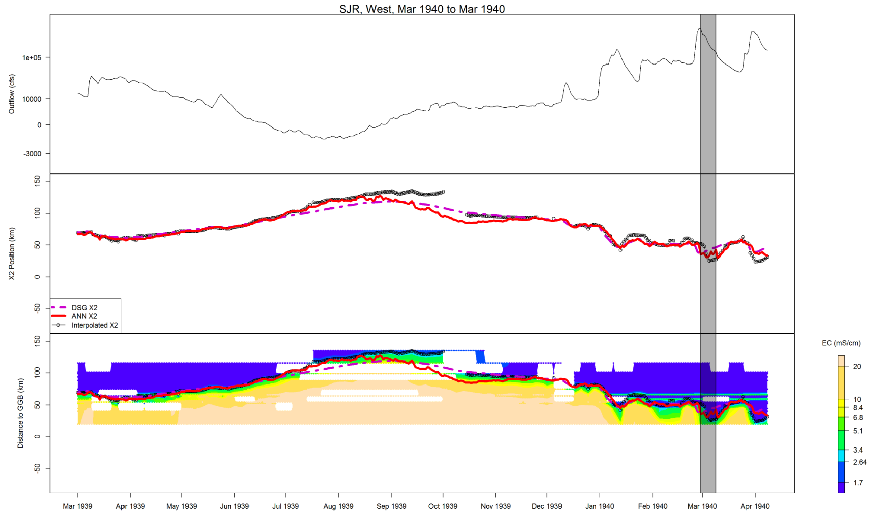
Figure B-29 Flow, X2, and salinity data for SJR, West, Mar 1940 to Mar 1940
