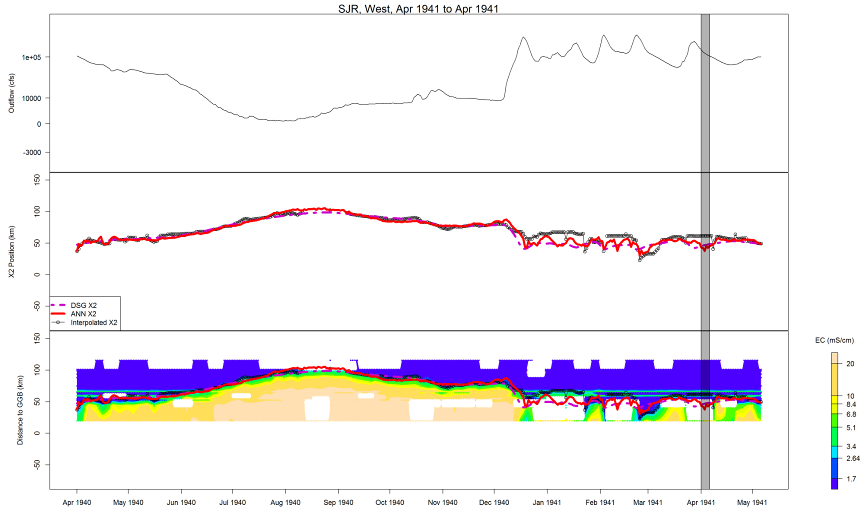
Figure B-31 Flow, X2, and salinity data for SJR, West, Apr 1941 to Apr 1941
