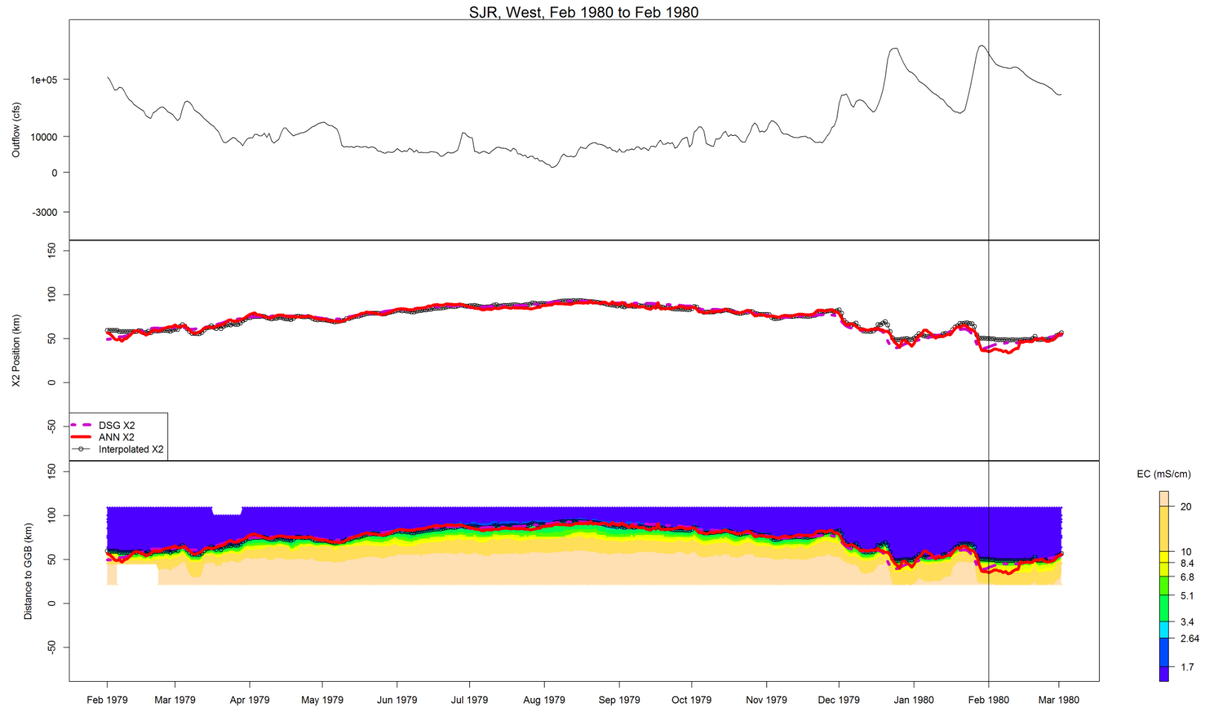
Figure B-41 Flow, X2, and salinity data for SJR, West, Feb 1980 to Feb 1980
