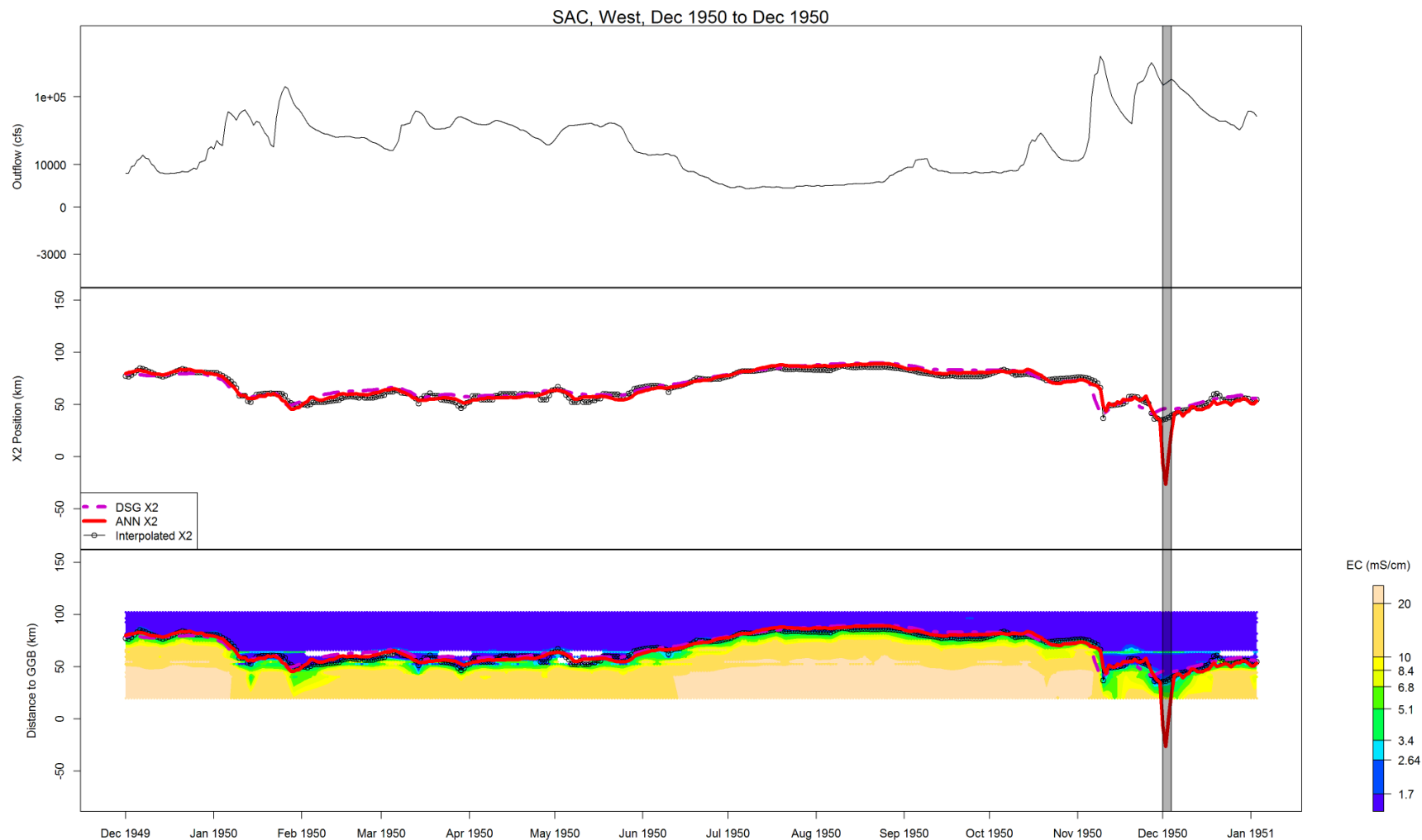
Figure B-8 Flow, X2, and salinity data for SAC, West, Dec 1950 to Dec 1950
