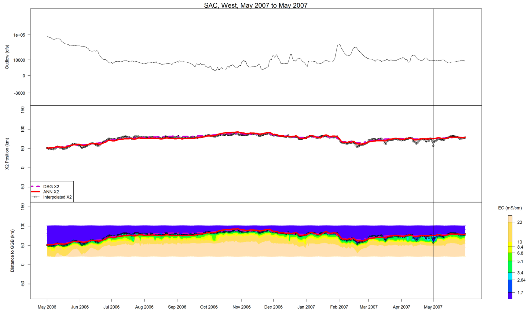
Figure B-19 Flow, X2, and salinity data for SAC, West, May 2007 to May 2007
