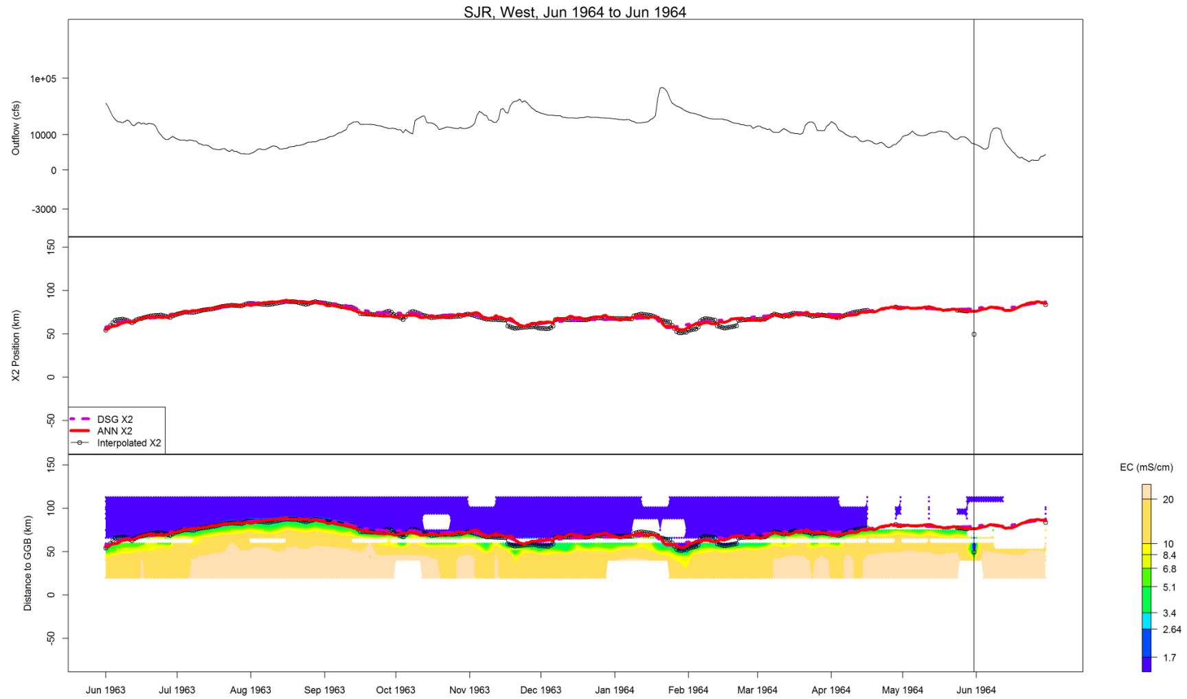
Figure B-39 Flow, X2, and salinity data for SJR, West, Jun 1964 to Jun 1964
