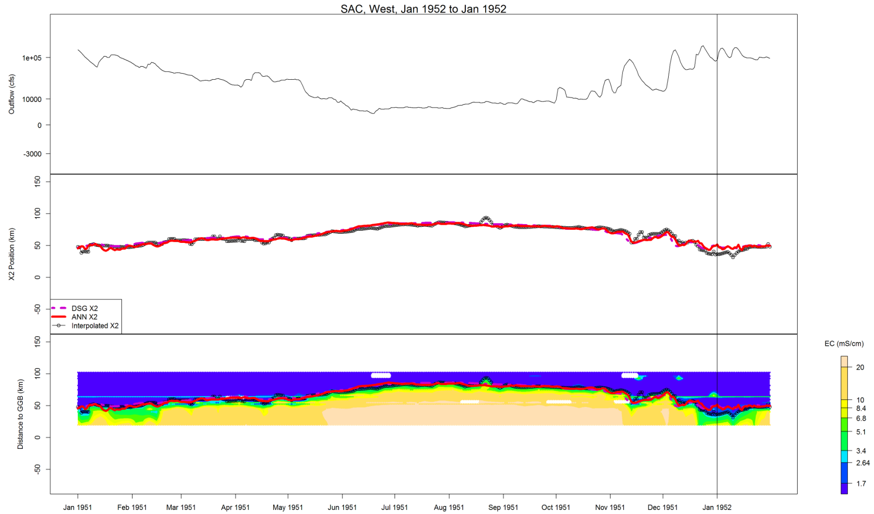
Figure B-9 Flow, X2, and salinity data for SAC, West, Jan 1952 to Jan 1952
