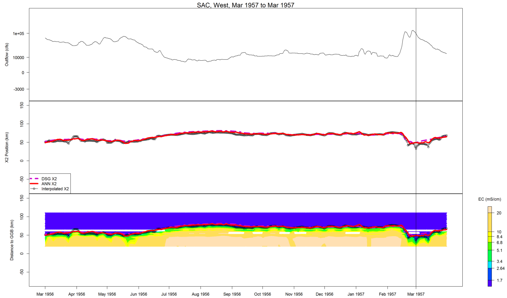
Figure B-13 Flow, X2, and salinity data for SAC, West, Mar 1957 to Mar 1957
