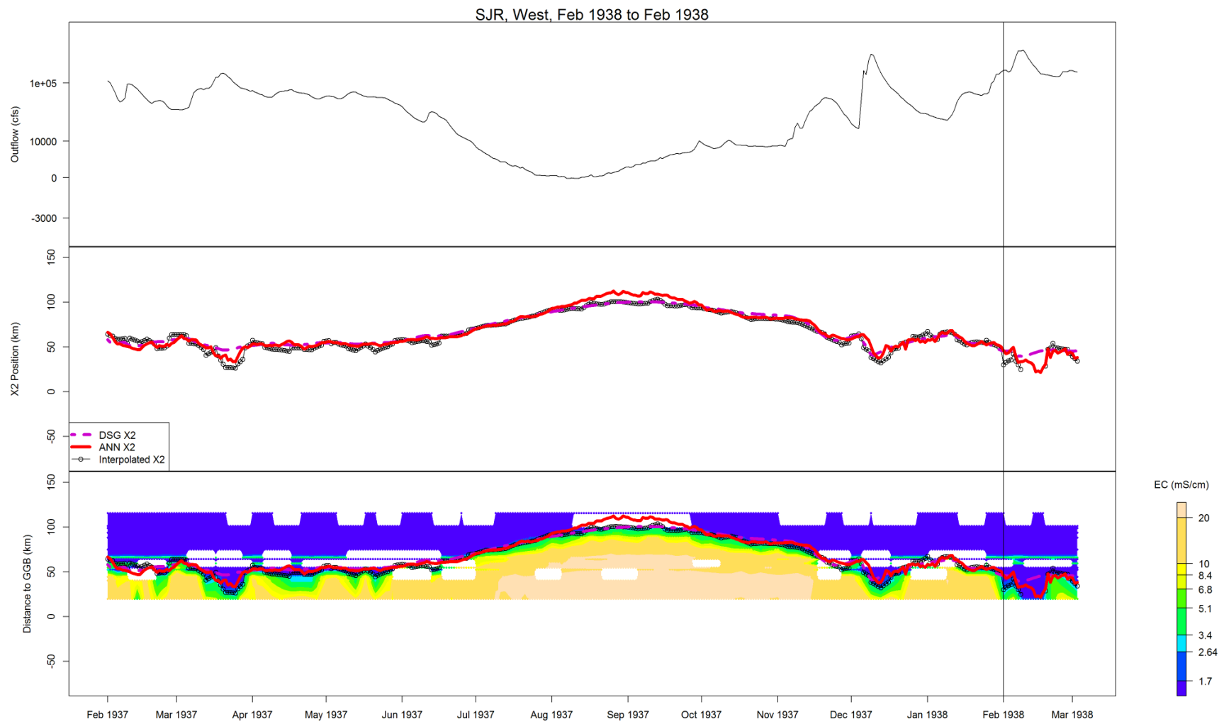
Figure B-26 Flow, X2, and salinity data for SJR, West, Feb 1938 to Feb 1938
