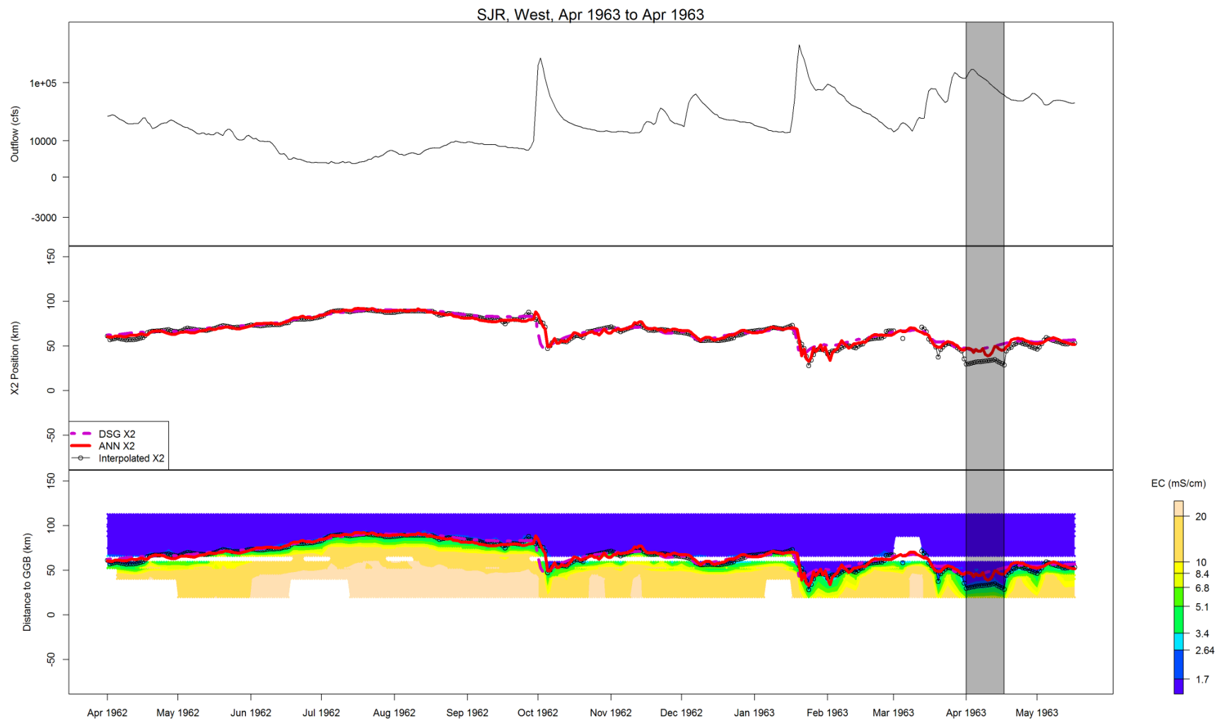
Figure B-38 Flow, X2, and salinity data for SJR, West, Apr 1963 to Apr 1963
