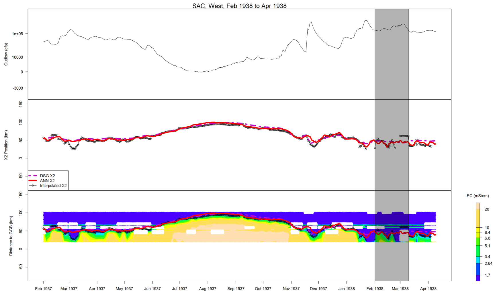
Figure B-4 Flow, X2, and salinity data for SAC, West, Feb 1938 to Apr 1938
