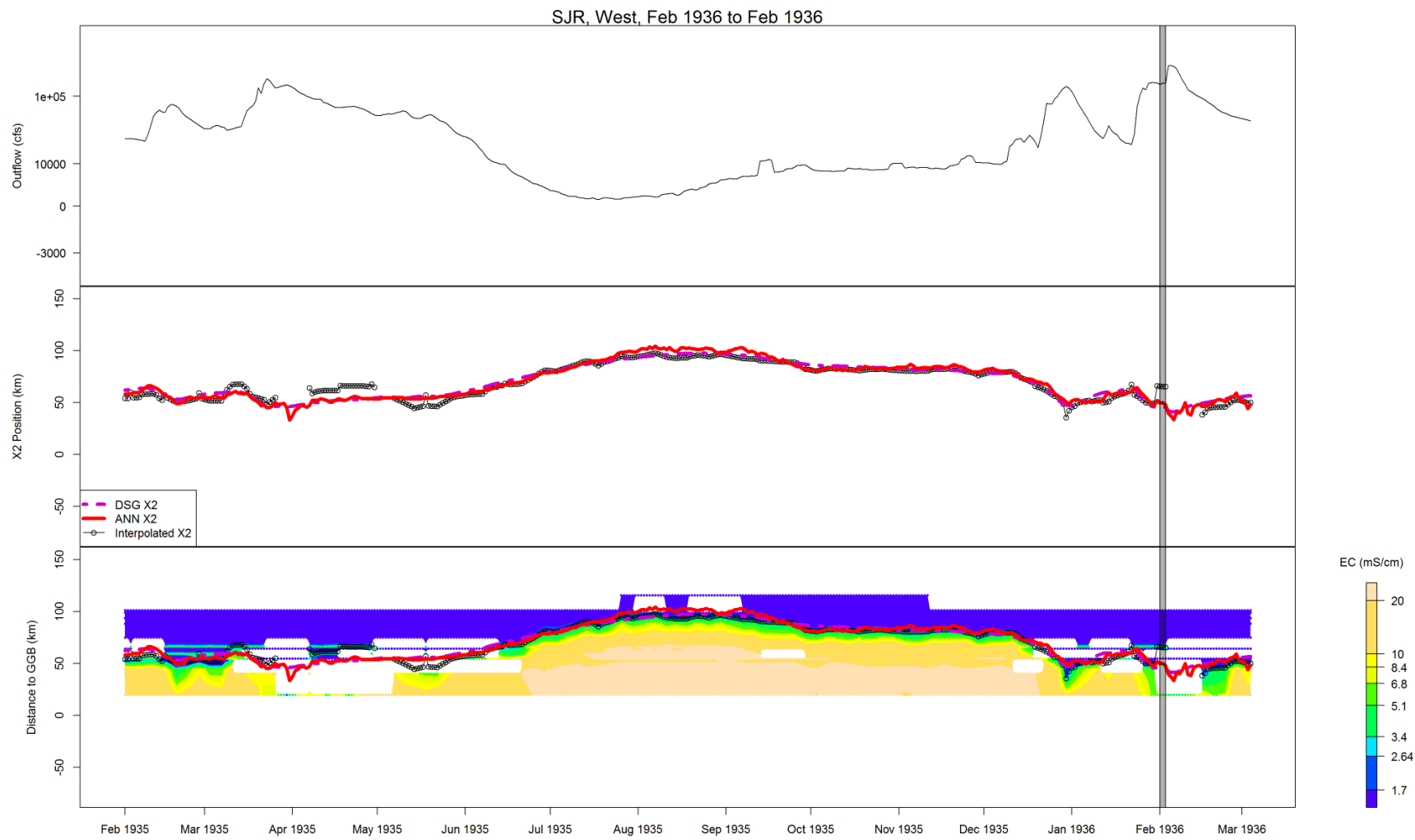
Figure B-24 Flow, X2, and salinity data for SJR, West, Feb 1936 to Feb 1936
