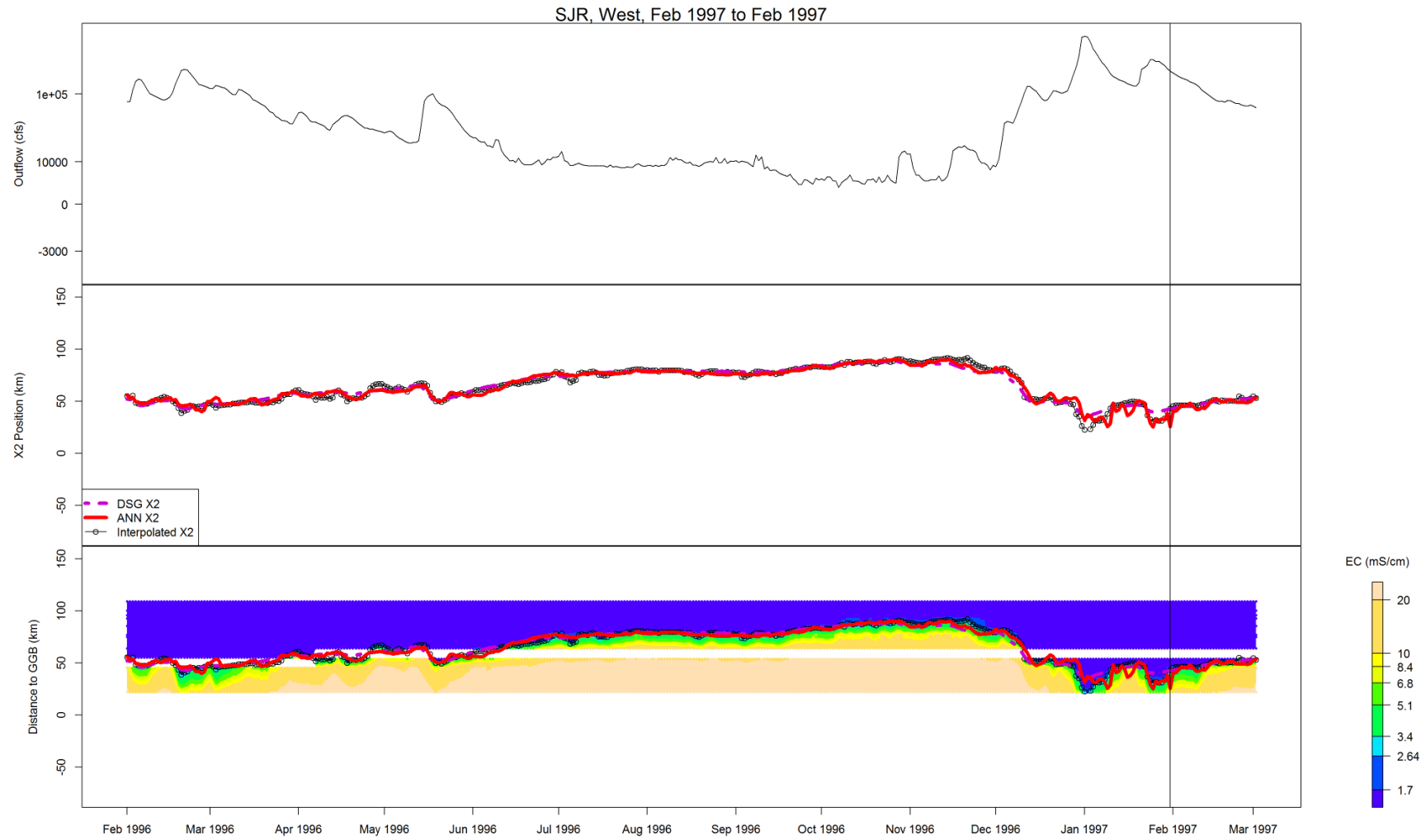
Figure B-43 Flow, X2, and salinity data for SJR, West, Feb 1997 to Feb 1997
