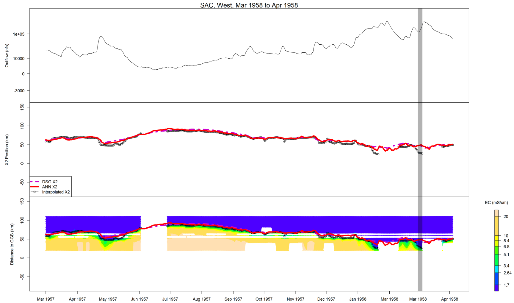
Figure B-15 Flow, X2, and salinity data for SAC, West, Mar 1958 to Apr 1958
