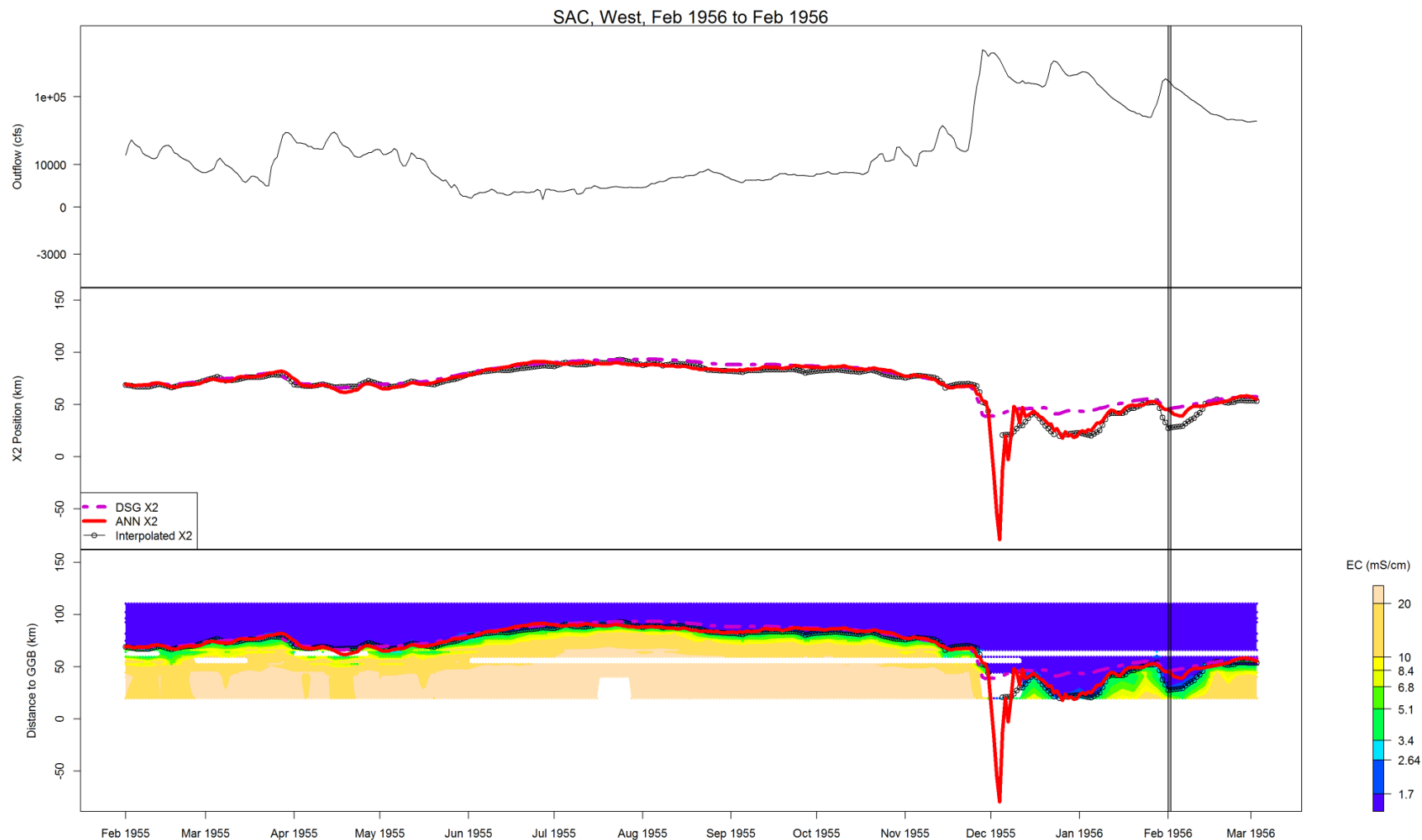
Figure B-12 Flow, X2, and salinity data for SAC, West, Feb 1956 to Feb 1956
