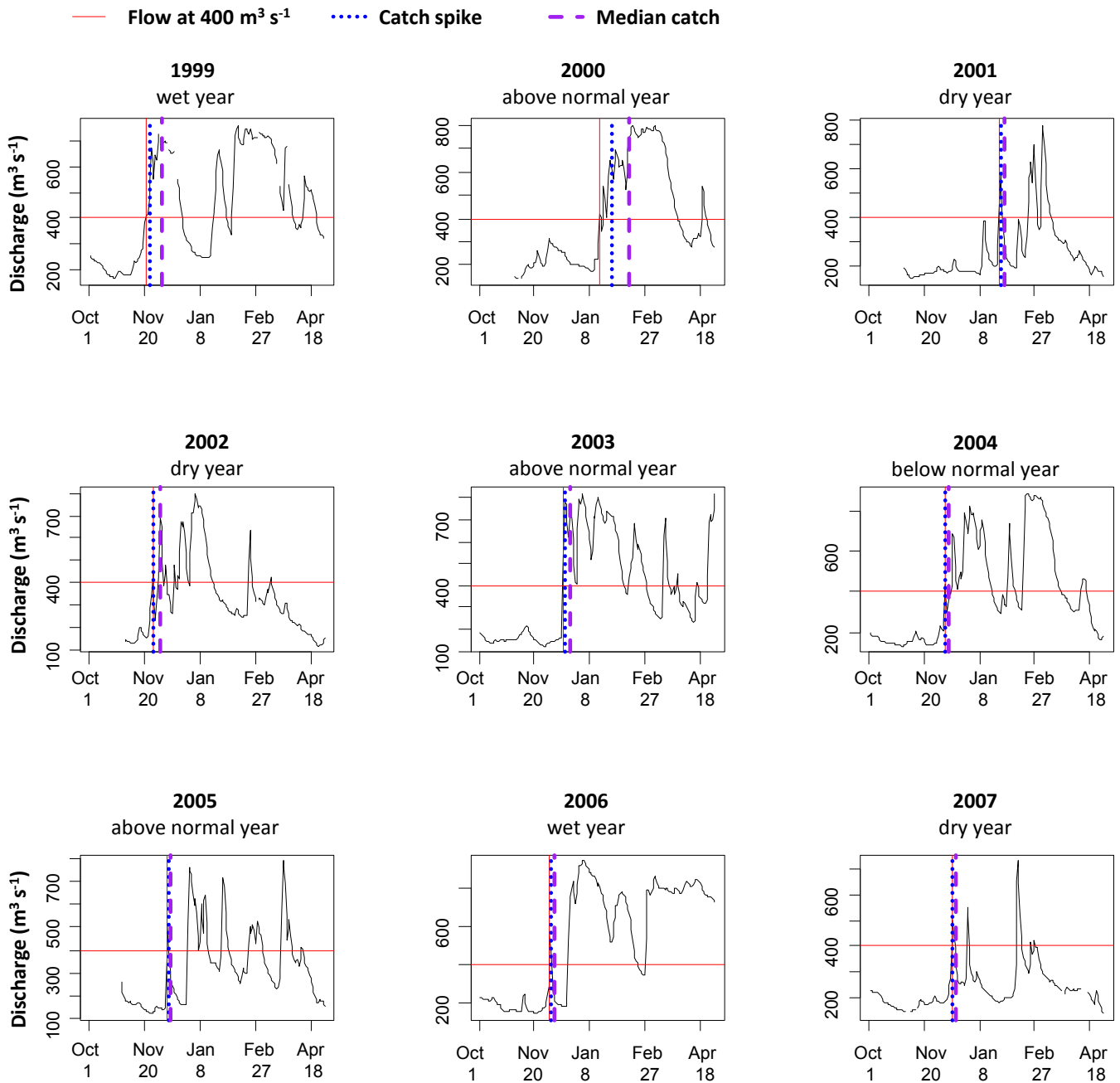
Figure 5 Flow threshold of 400 m³ s⁻¹ triggers abrupt and substantial winter-run migration into the Delta at Knights Landing. The first day that flows reached 400 m³ s⁻¹ (solid vertical line) is nearly coincident with the day of catch spike (increase of 5% of cumulative catch; dotted line) and the day of median catch (50th percentile of cumulative catch; dashed line). Years refer to spring emigration season.
