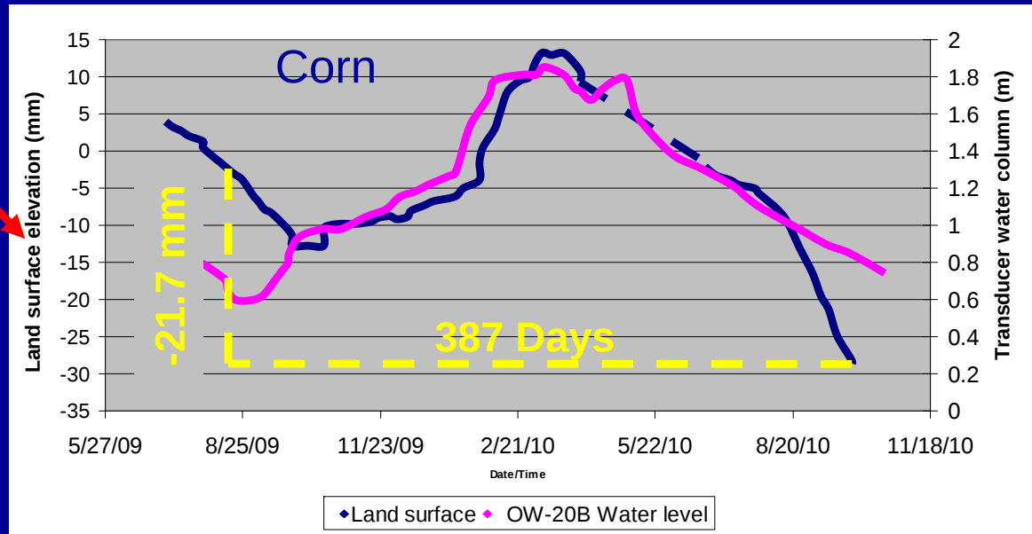
Land-Surface Elevation and Groundwater levels at corn field extensometer
