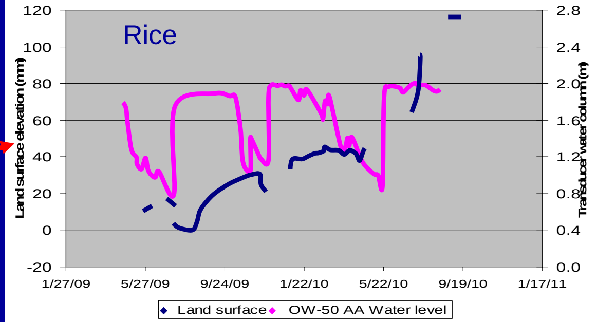
Land-Surface Elevation and Groundwater levels at rice field extensometer
